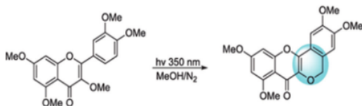
Figure 1: UV absorption by quercetin pentamethyl ether
